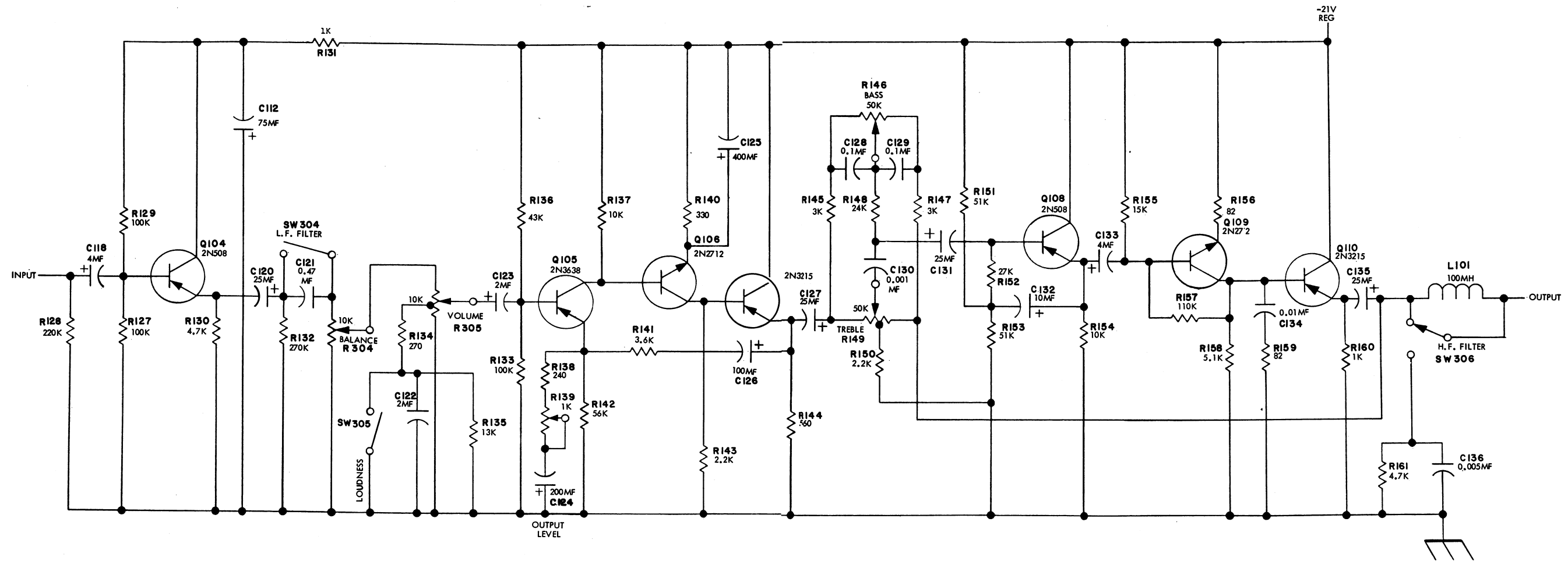
LINE AMPLIFIER
