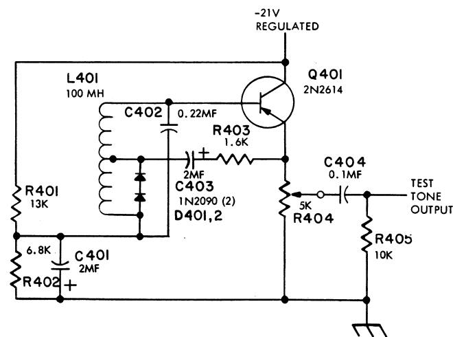
TONE OSCILLATOR
