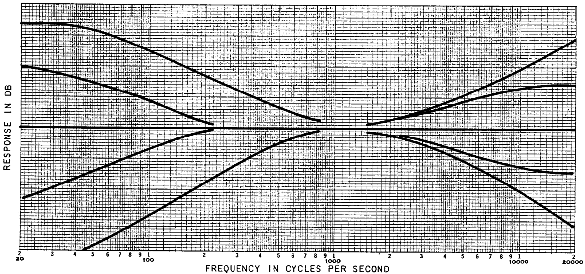
FIGURE 3-5 TONE CONTROL
